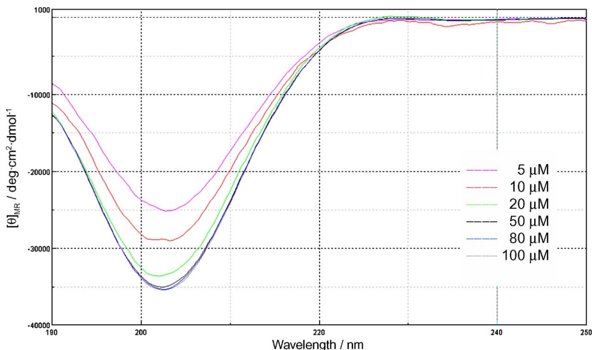
Fig. 5. CD spectra of SAP at varying concentrations ( c=5-100 \mu M) in 10 mM aq. phosphate buffer at pH 7.
